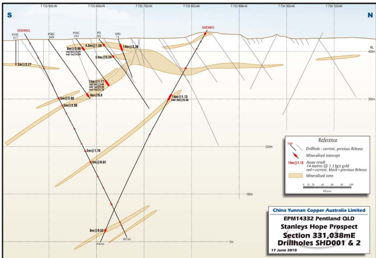
Figure 2: Section of SDH001 and SDH002. This interpretation will be revised after geological reinterpretation of previous drilling that is facilitated by the scout diamond drilling completed by CYU.
