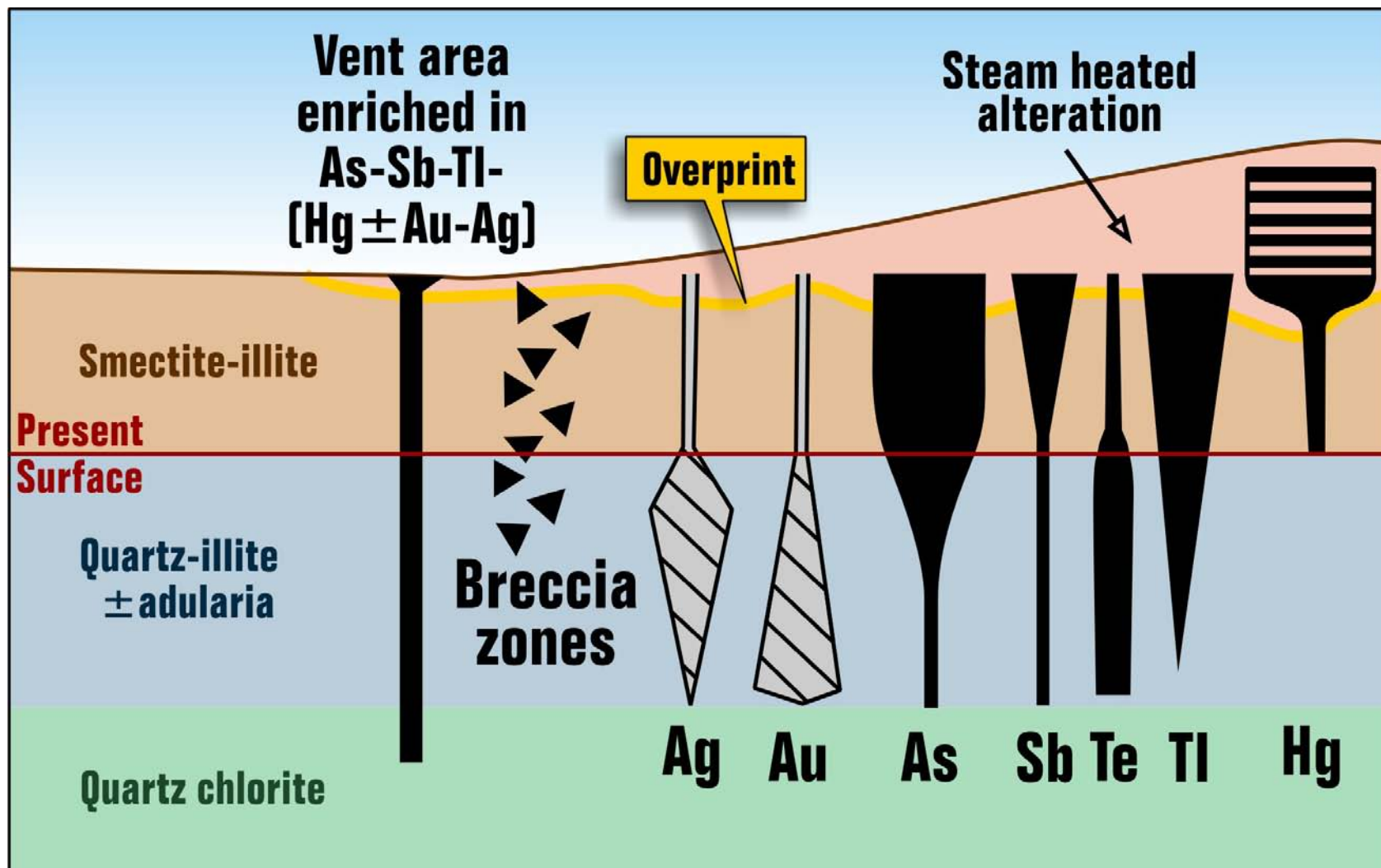
Figure 5: Schematic of Metal Zonation at Stanley's Hope. At the current level of erosion represented by the red line near surface we expect an increase in gold and silver grades with depth. As predicted by this diagram industry standard diagram for low sulphidation epithermals and associated alteration, Arsenic (As) and Antimony (Sb) are useful pathfinder elements.
